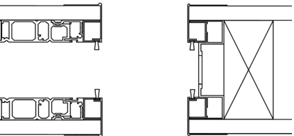
REBATED SQUARE-SET
