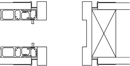
REBATED
