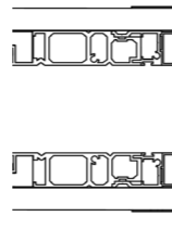
REBATED SQUARE-SET
