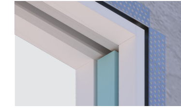
BULKHEAD SHADOWLINE
