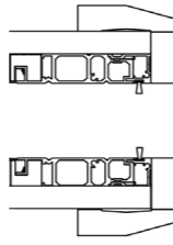
ARCHITRAVES
